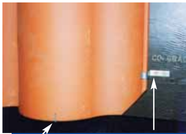
Perfect placement of Hurricane Side Clip
